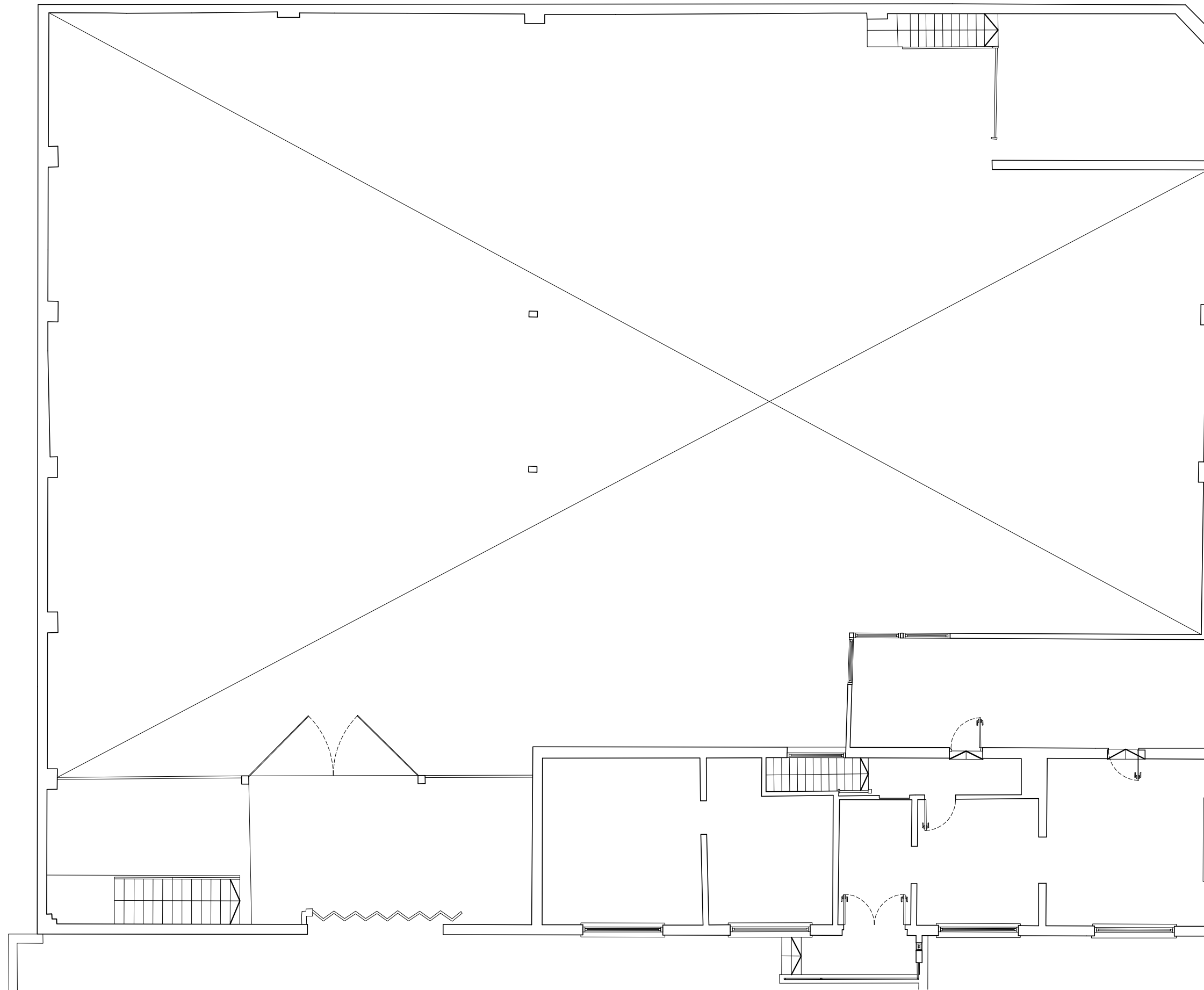
GROUND FLOOR PLAN SCALE 1:100 0 1 2 3 4 5m
